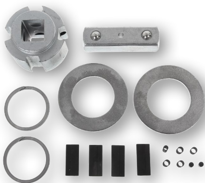
13215 Repair Kit
